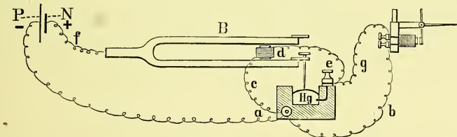
FIG. 11. DIAGRAM OF AN ARRANGEMENT OF A VIBRATING TUNING-FORK WITH A DESPRETZ SIGNAL.
